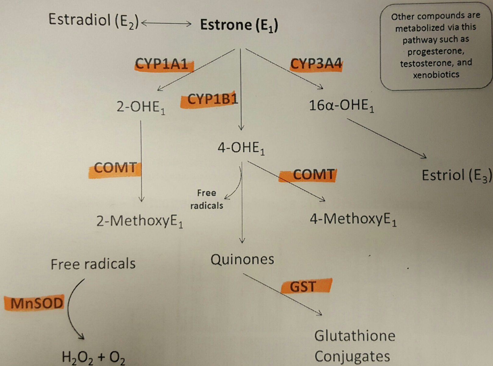
Figure 2 - Oxidative Metabolism of Estrogens
